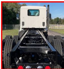
Chassis Layout
